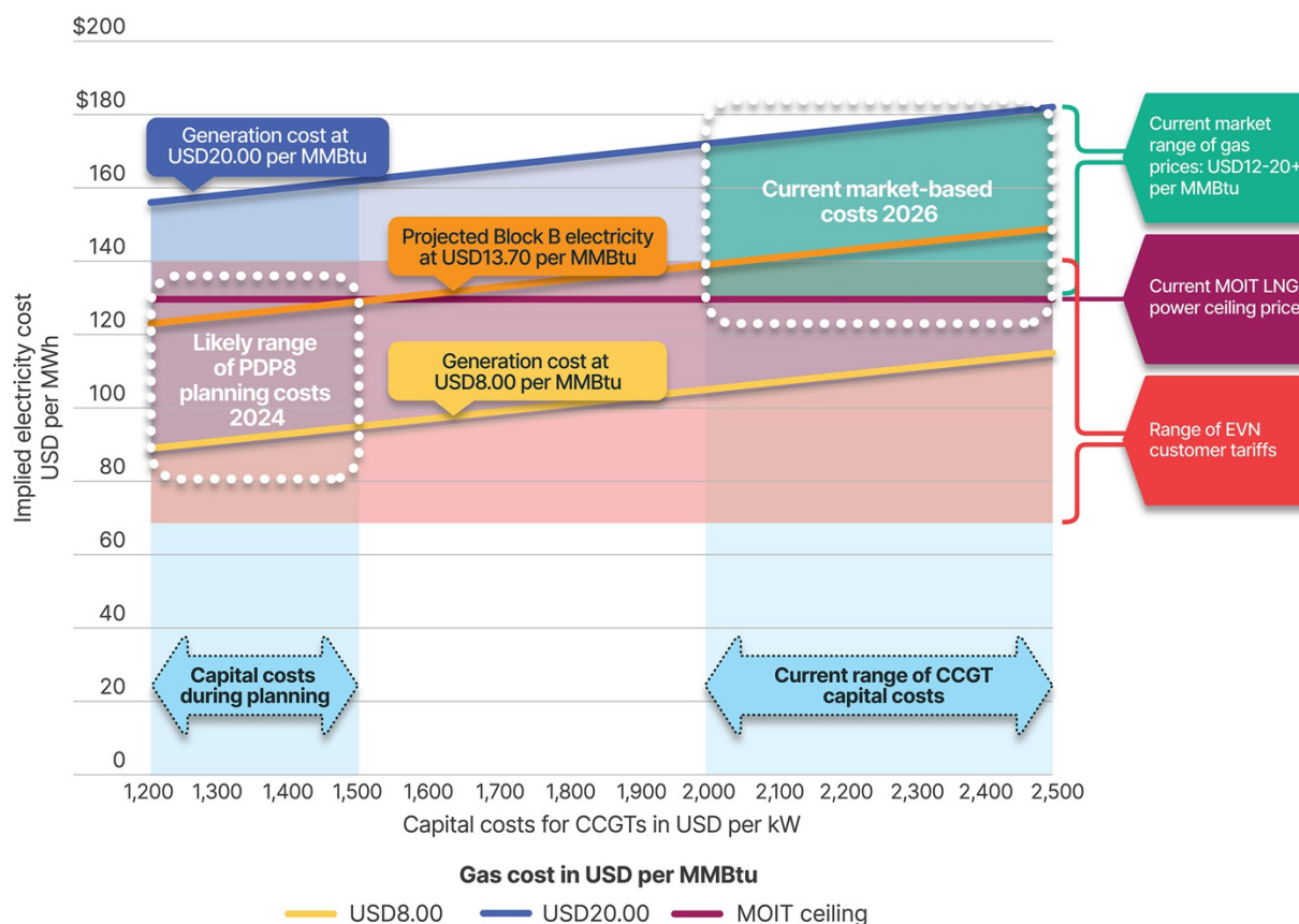
Figure 5: Modeled electricity cost across a range of CCGT capital costs and LNG prices
