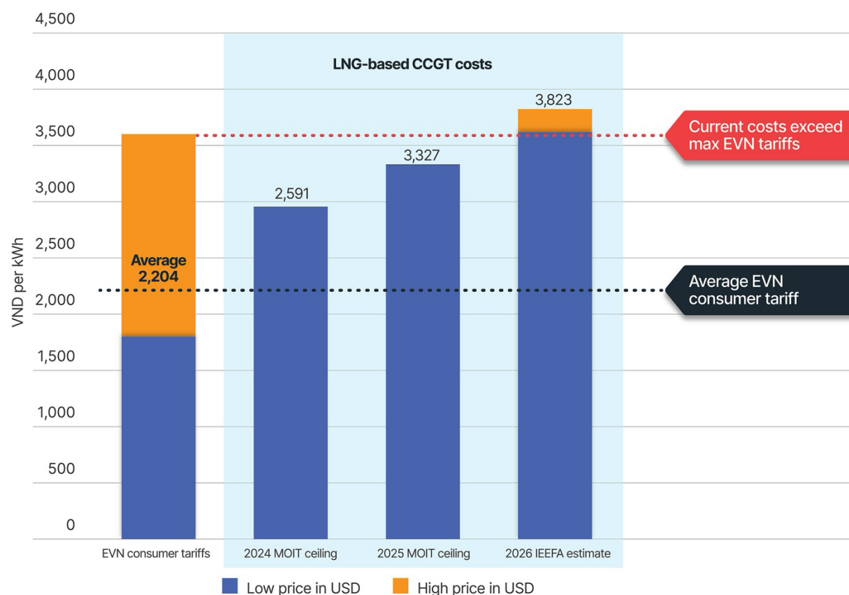
Figure 4: Comparison of EVN consumer tariffs to LNG generation costs
