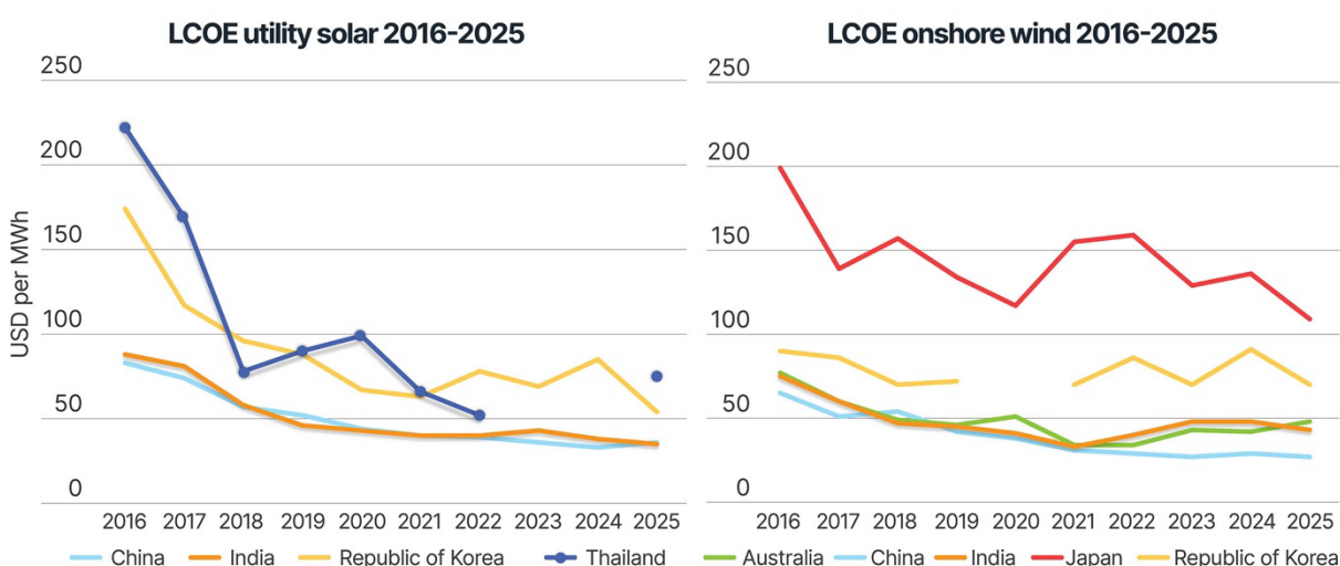
Figure 6: IRENA comparable market costs for solar and wind energy, 2016 to 2025
