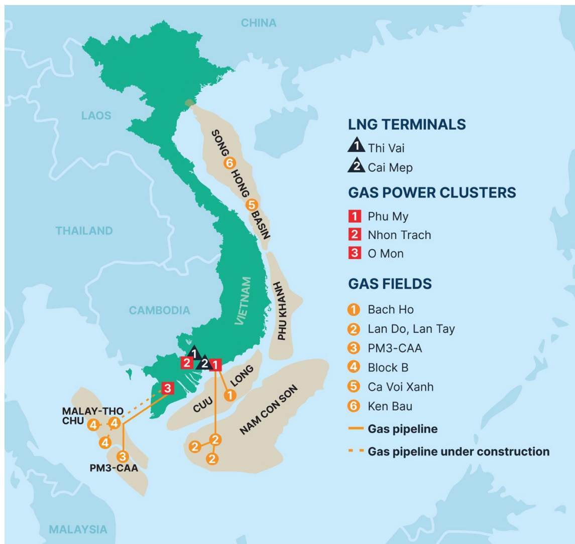
Figure 2: Vietnam's gas fields, gas infrastructure, and downstream consumption centers
