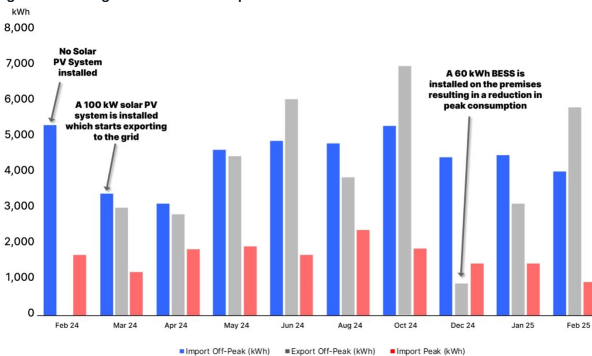
Figure 16: Changes in Peak Consumption after Installation of Solar + BESS at Gem Net
