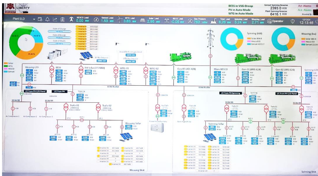
Figure 19: EMS System Dashboard at LML
