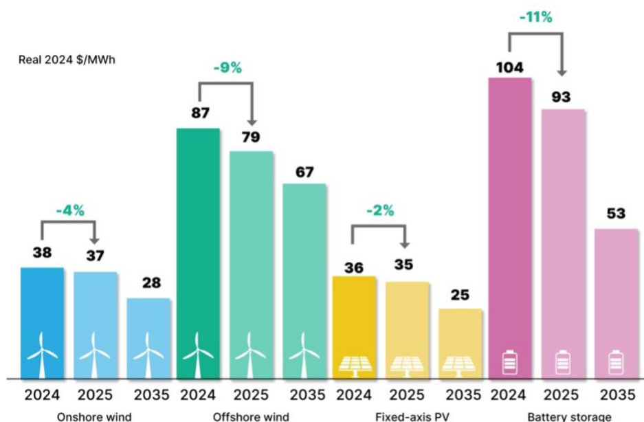
Figure 7: BNEF's LCOE Outlook for Battery Storage Clean Energy Technologies, 2024, 2025, 2035
