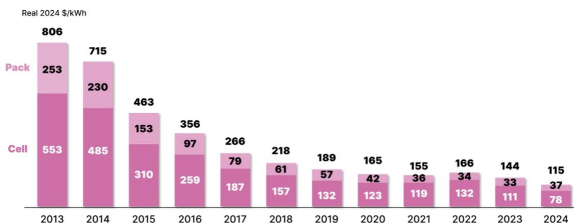
Figure 6: Volume-weighted Average Lithium-ion Battery Pack and Cell Prices, 2013-2024
