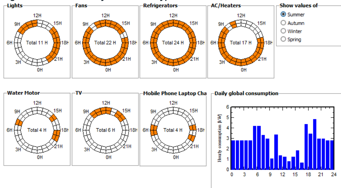
Figure 8: Summer Hourly Profile of a Typical 10kW Sanctioned Load Consumer
