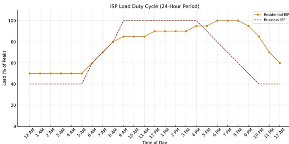
Figure 14: Typical Load Duty Cycle of an ISP
