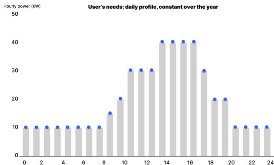
Figure 11: Typical Load Profile of a Commercial Establishment
