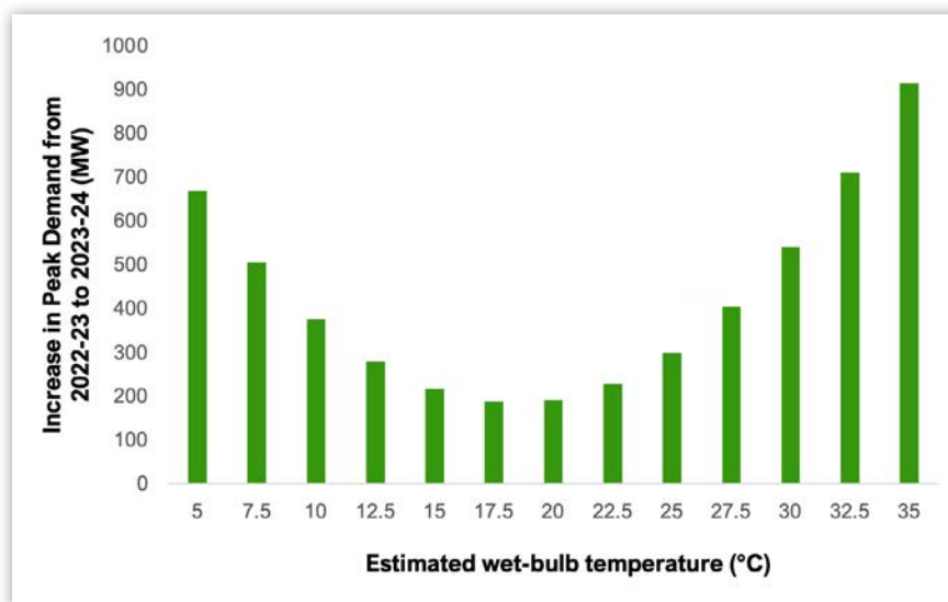
Figure 2: Delhi’s Peak Demand Increase at 13 Different WBTs
