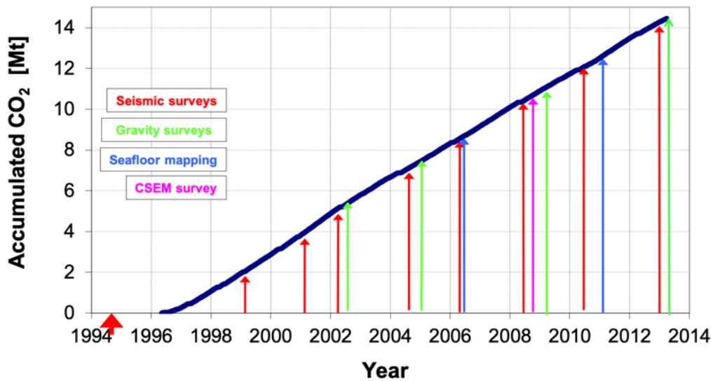
Figure 10: Sleipner CCS Injection and Monitoring History (1994–2014)
