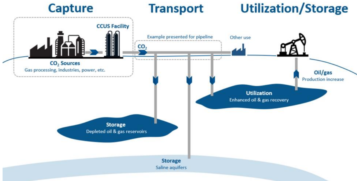
Figure 1: CCUS Schematics
