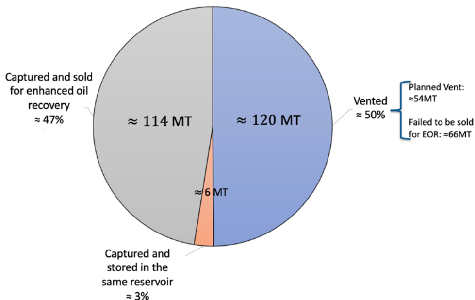
Figure 7: Shute Creek CCUS Lifetime CO 2 Capture Performance
