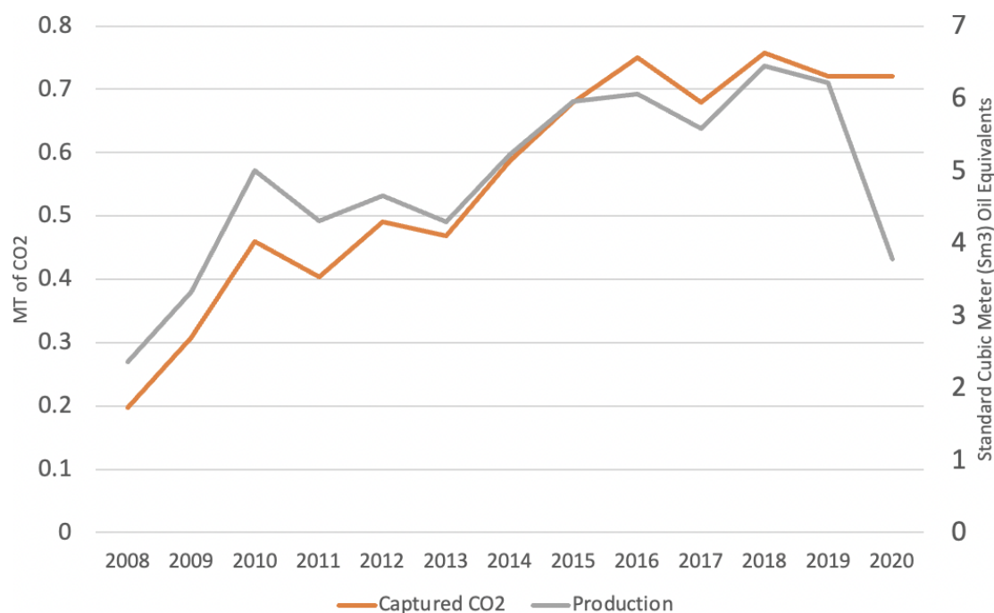
Figure 11: Snøhvit Project: Production vs Captured CO 2
