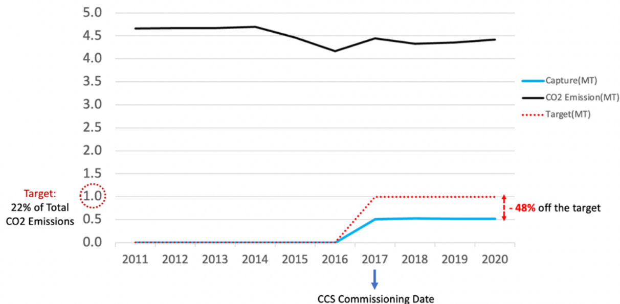
Figure 22: CO 2 Emissions vs Capture Performance of the IL-CCS Plant (2011–2020)
