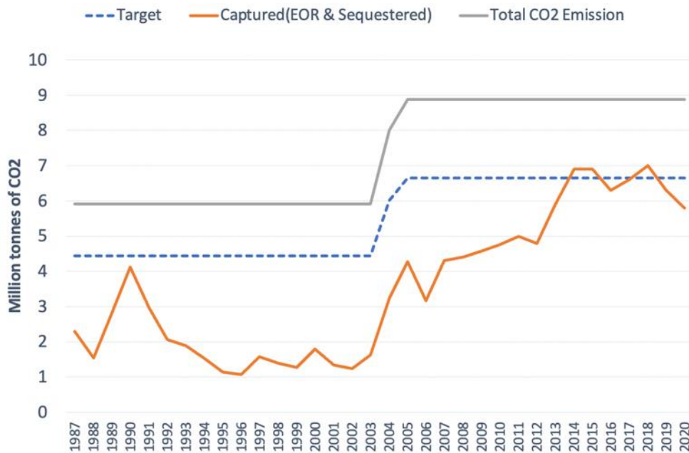
Figure 6: Capturing Performance Trend of the Shute Creek CCUS Plant (1987–2020)
