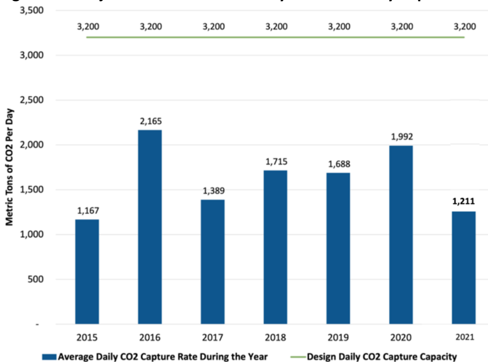
Figure 16: Projected vs Actual Boundary Dam CO 2 Daily Capture Rate
