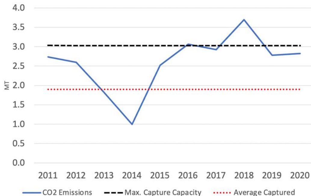
Figure 20: Great Plains Synfuels Plant CO 2 Emissions vs Capture Performance (2011–2020)
