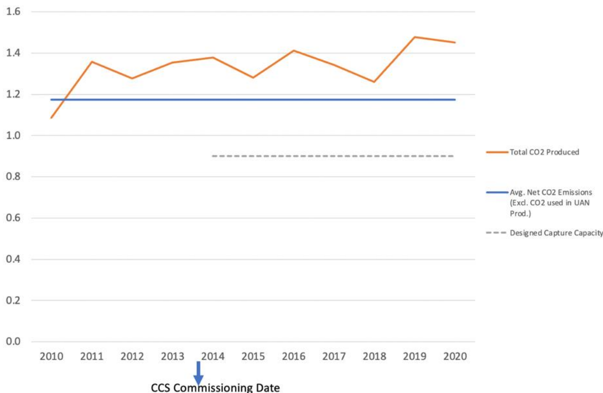
Figure 23: Coffeyville CCS CO 2 Emissions vs Maximum Capturing Capacity (2010–2020)
