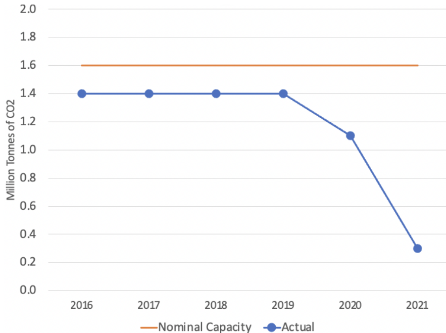
Figure 12: Snøhvit and Sleipner Projects: Carbon Capture Performance (2016–2021)
